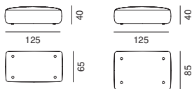
seating module M
